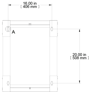
REAR VIEW WALL MOUNT DIMENSIONS
