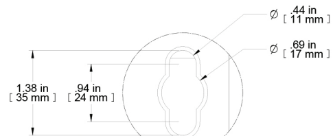
DETAIL A MOUNTING HOLES TYP 4 PLACES
